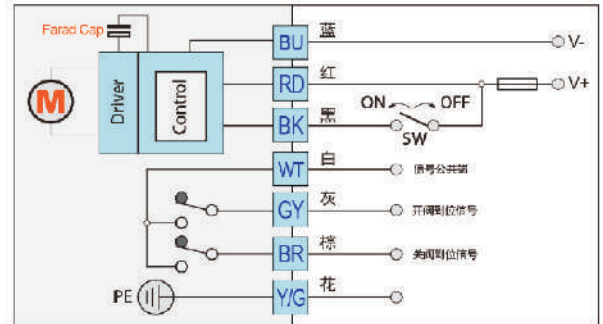
开关型-断电复位接线指示 KT32S/BD3S (DC)
