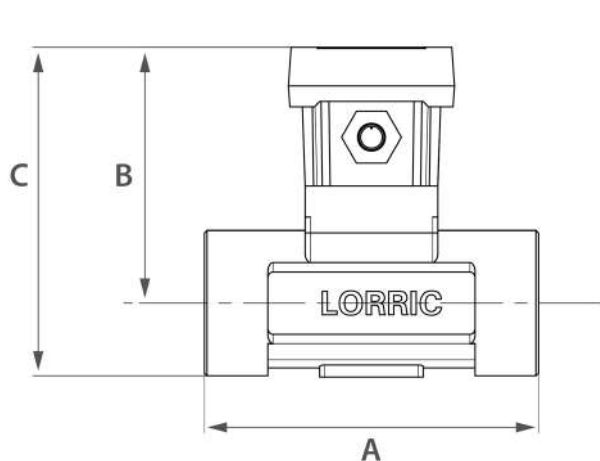
Stainless steel - Female Thread
