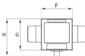
DN-20 (3/4") Stainless steel - Male Thread
